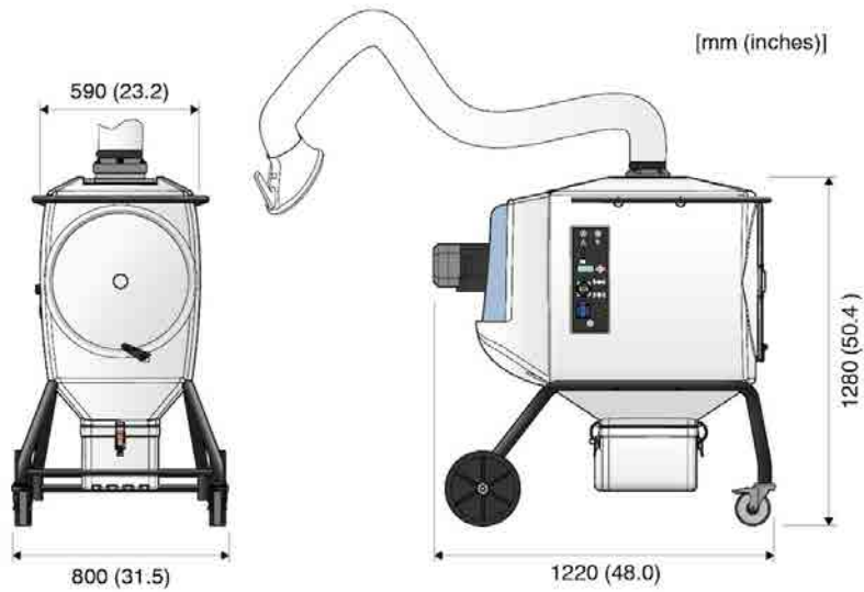
Mobile FilterBox Hygiene 12A
