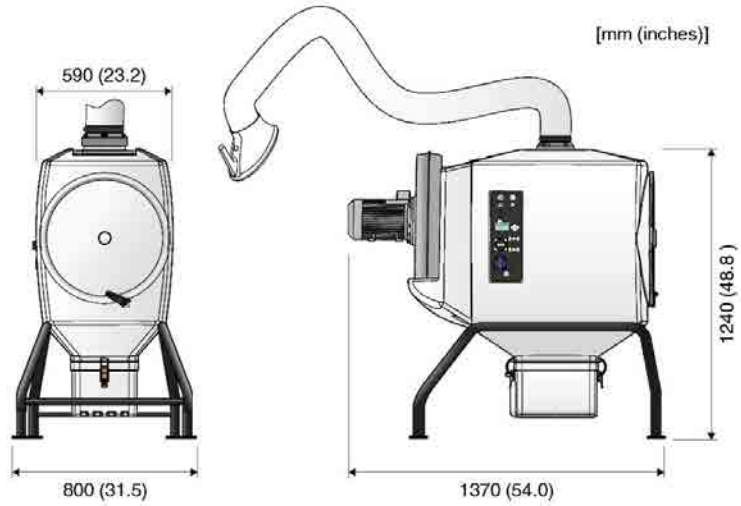
Floor mounted FilterBox Hygiene 12A
